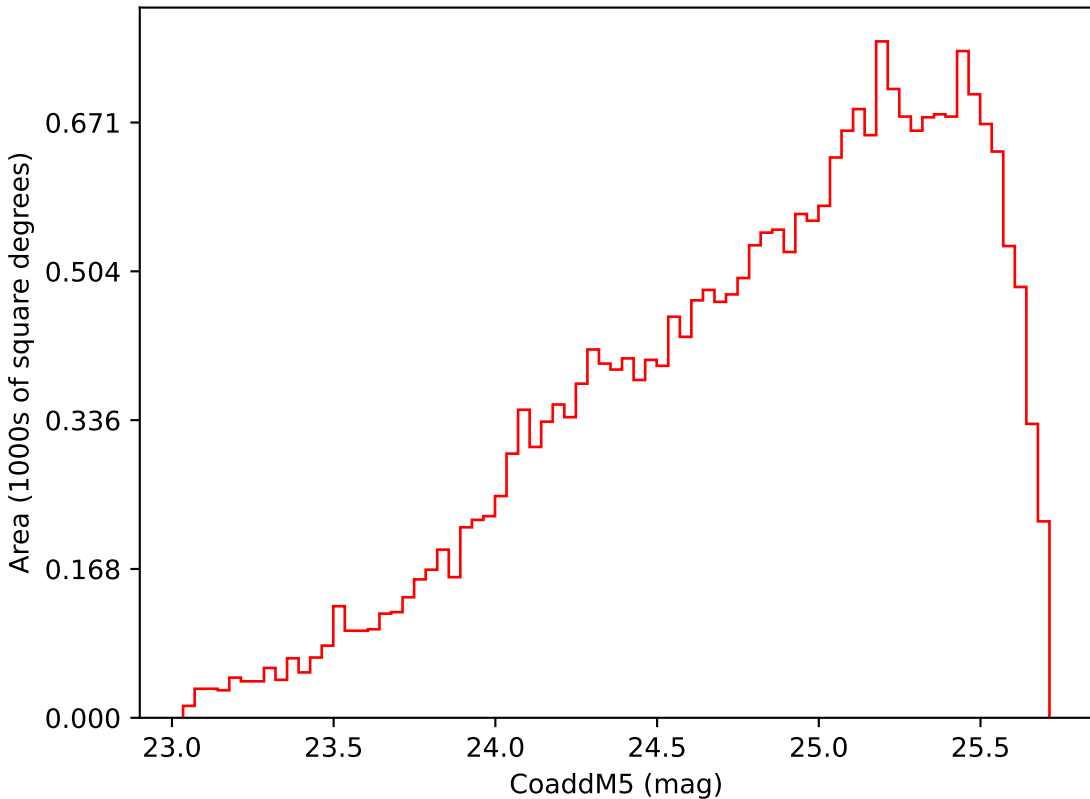
ddf_loaded_fl8_v3.4_10yrs Yr 3-4 i band: CoaddM5
