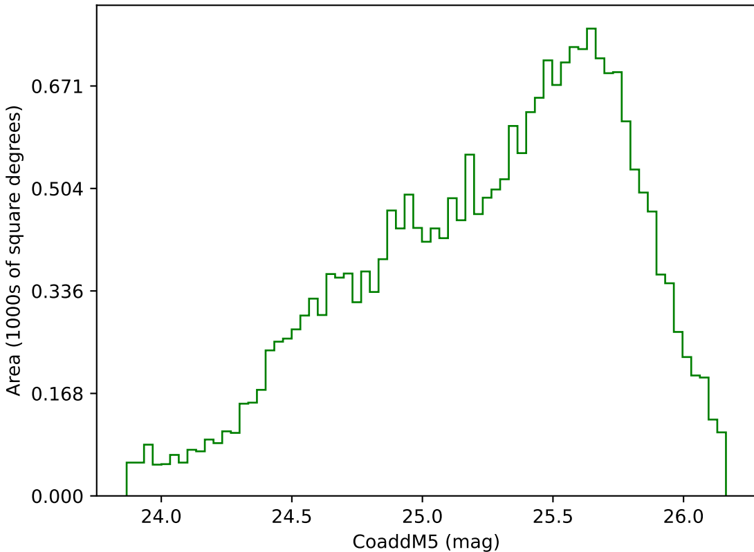
ddf_loaded_fl8_v3.4_10yrs Yr 3-4 g band: CoaddM5
