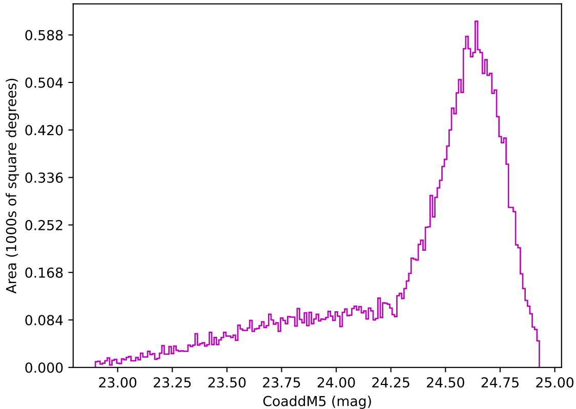
ddf_loaded_fl8_v3.4_10yrs Yr 1 z band: CoaddM5
