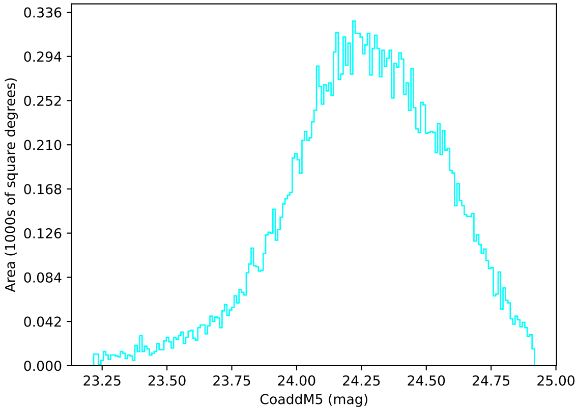
ddf_loaded_fl8_v3.4_10yrs Yr 1 u band: CoaddM5
