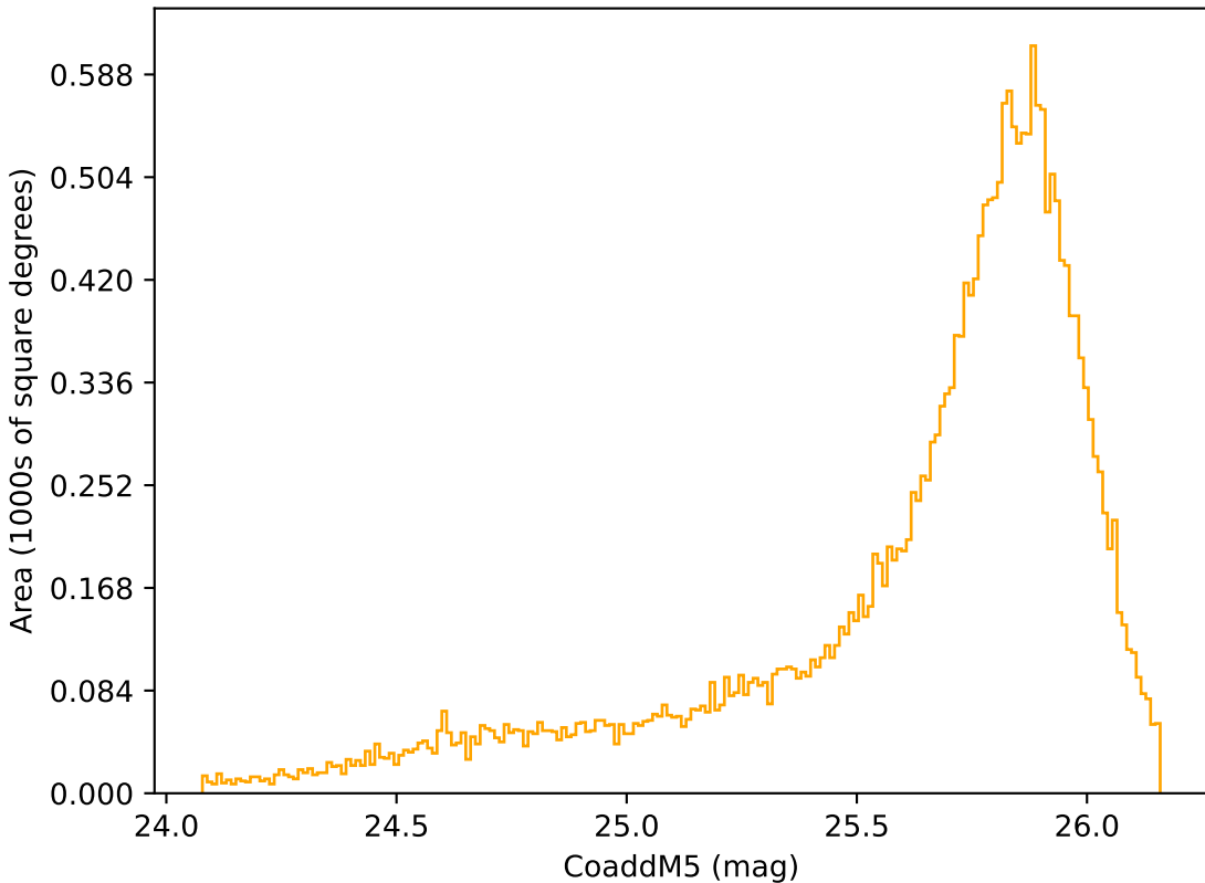
ddf_loaded_fl8_v3.4_10yrs Yr 1 r band: CoaddM5
