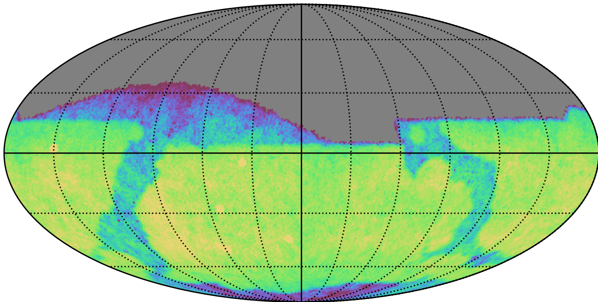
ddf_loaded_fl8_v3.4_10yrs Yr 1 i band: CoaddM5
