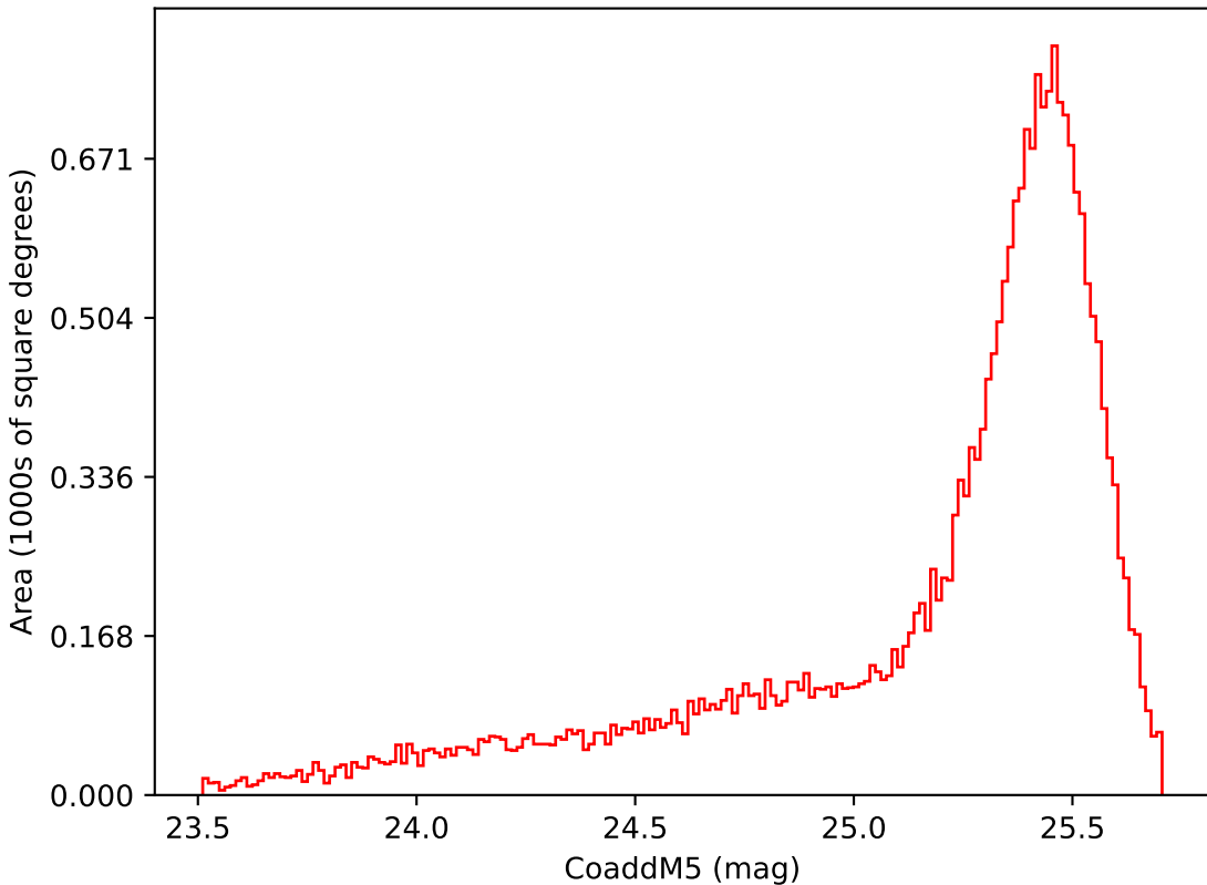
ddf_loaded_fl8_v3.4_10yrs Yr 1 i band: CoaddM5
