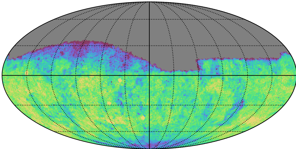
ddf_loaded_fl8_v3.4_10yrs Yr 1 g band: CoaddM5
