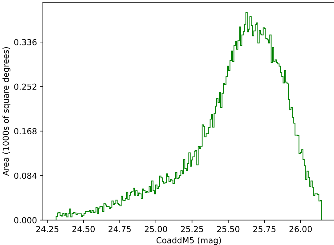
ddf_loaded_fl8_v3.4_10yrs Yr 1 g band: CoaddM5
