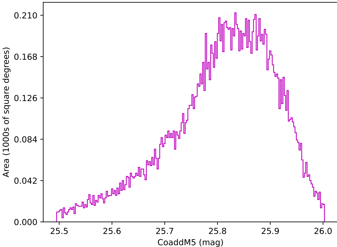
ddf_loaded_fl8_v3.4_10yrs WFD z band: CoaddM5
