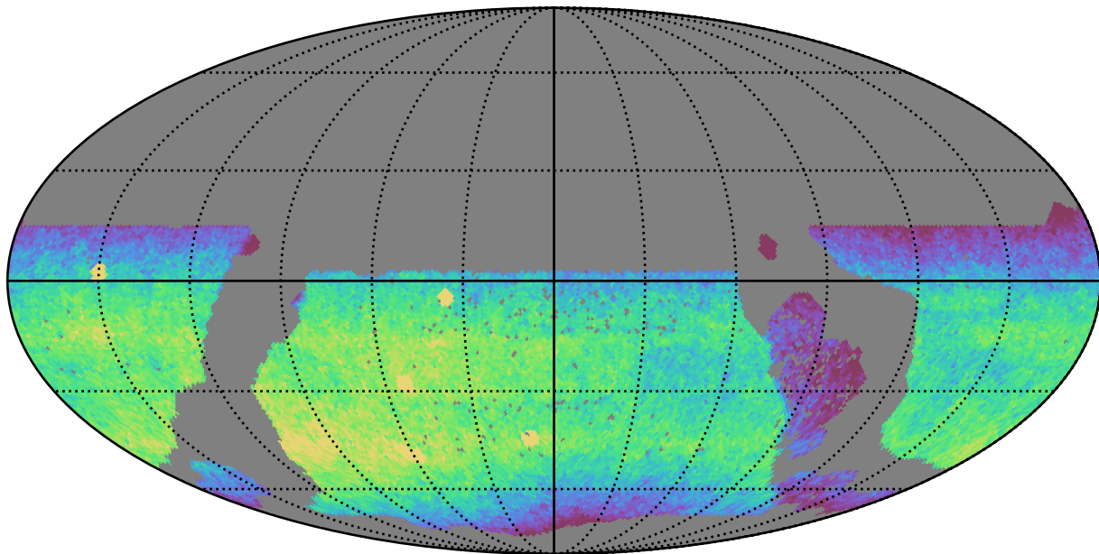
ddf_loaded_fl8_v3.4_10yrs WFD y band: CoaddM5
