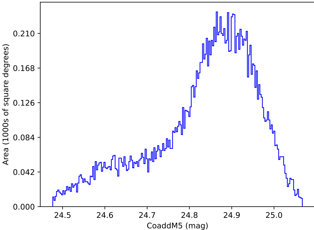
ddf_loaded_fl8_v3.4_10yrs WFD y band: CoaddM5
