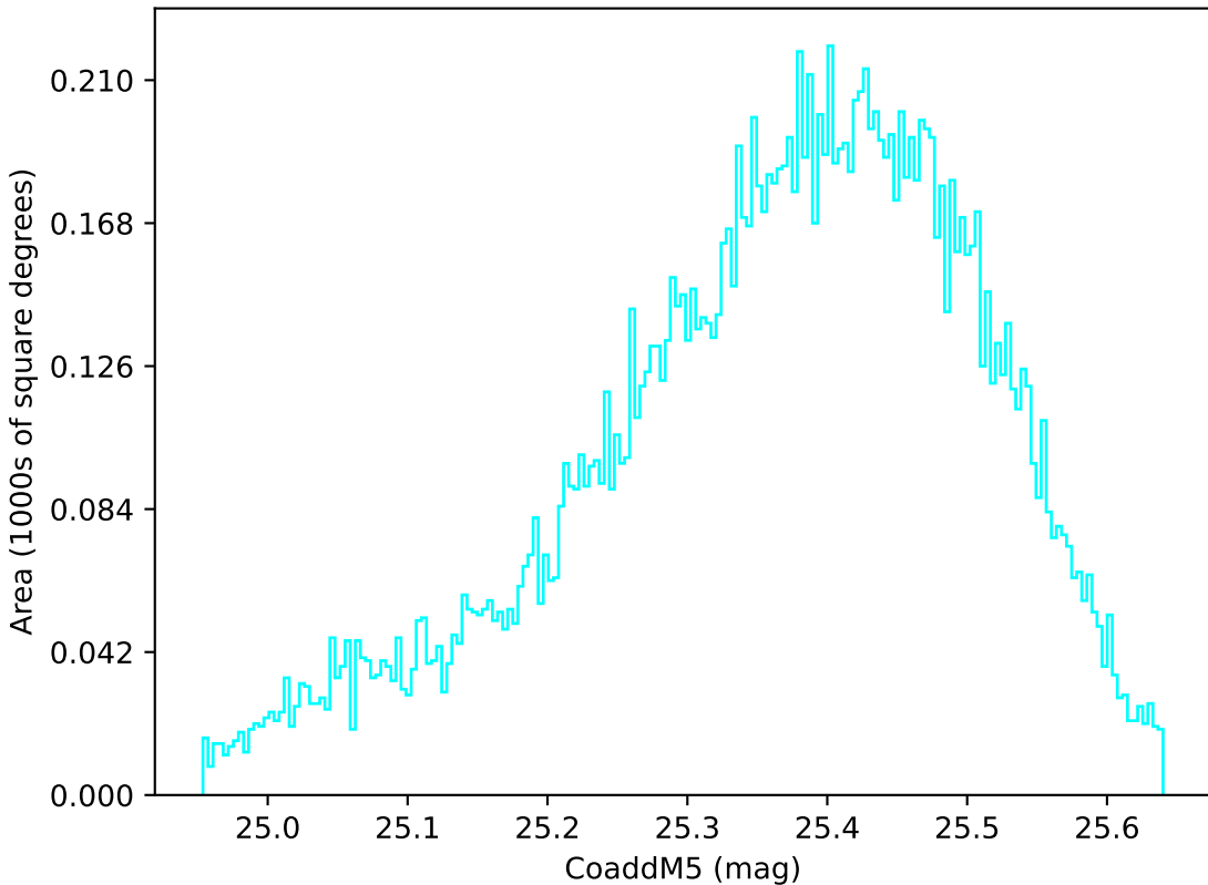
ddf_loaded_fl8_v3.4_10yrs WFD u band: CoaddM5
