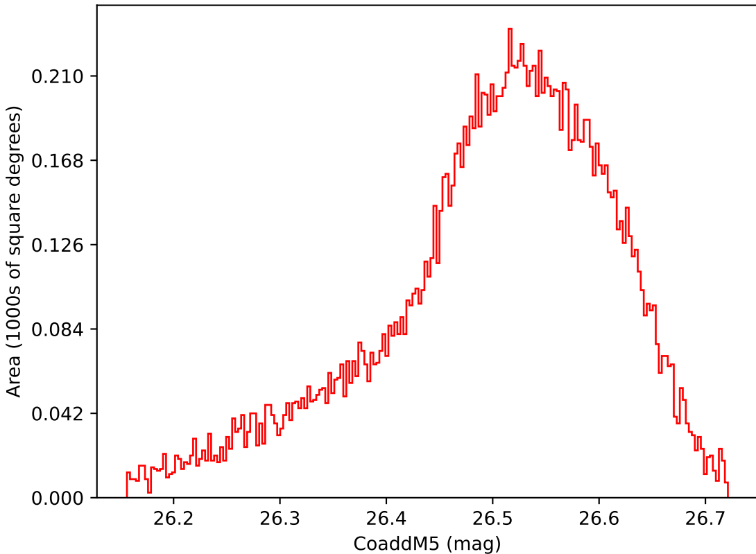
ddf_loaded_fl8_v3.4_10yrs WFD i band: CoaddM5
