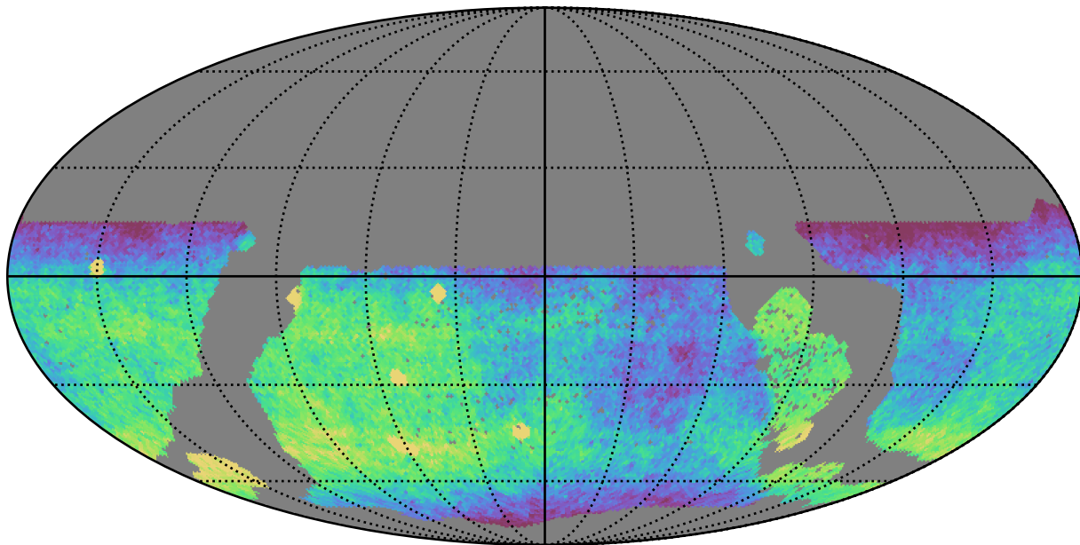
ddf_loaded_fl8_v3.4_10yrs WFD g band: CoaddM5
