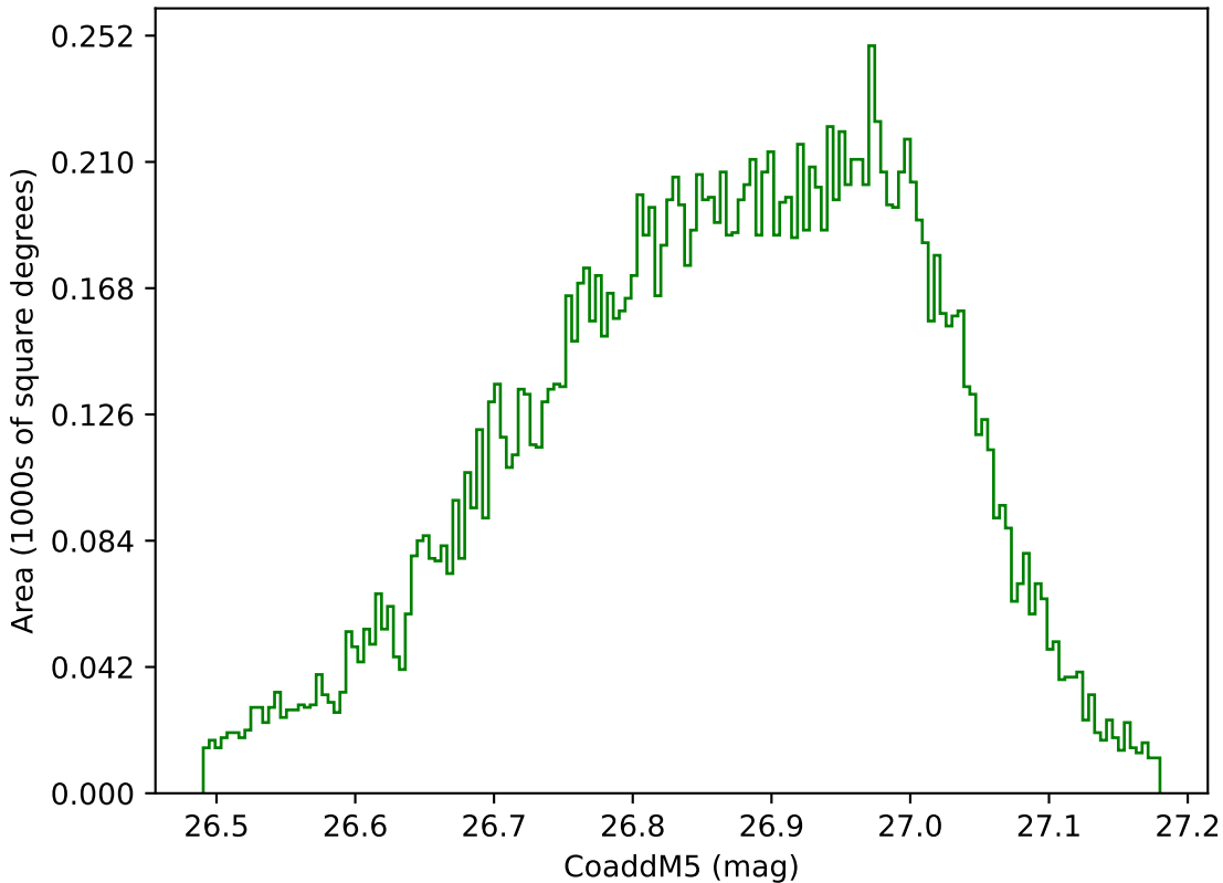
ddf_loaded_fl8_v3.4_10yrs WFD g band: CoaddM5
