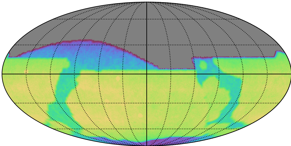
ddf_loaded_fl8_v3.4_10yrs All sky z band: CoaddM5
