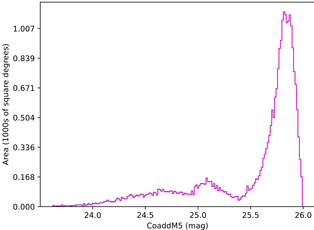
ddf_loaded_fl8_v3.4_10yrs All sky z band: CoaddM5
