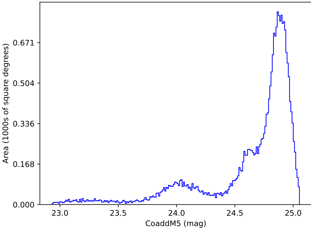
ddf_loaded_fl8_v3.4_10yrs All sky y band: CoaddM5
