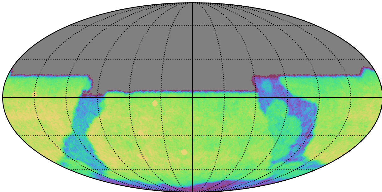
ddf_loaded_fl8_v3.4_10yrs All sky u band: CoaddM5
