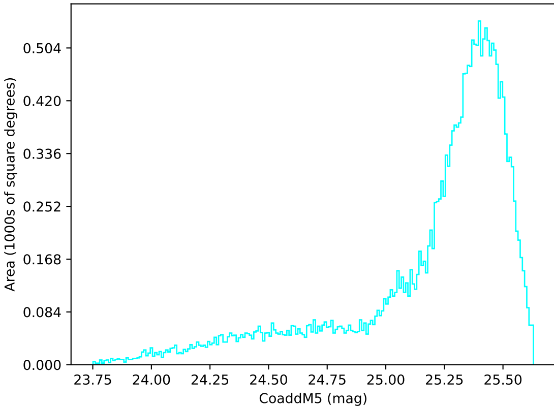
ddf_loaded_fl8_v3.4_10yrs All sky u band: CoaddM5
