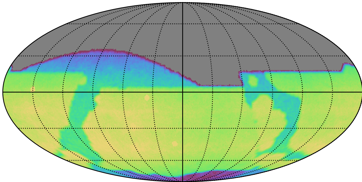
ddf_loaded_fl8_v3.4_10yrs All sky r band: CoaddM5
