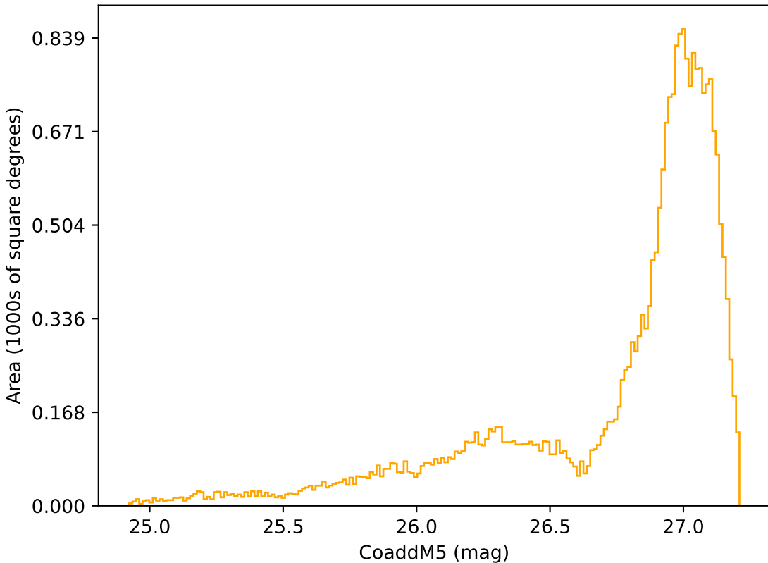
ddf_loaded_fl8_v3.4_10yrs All sky r band: CoaddM5
