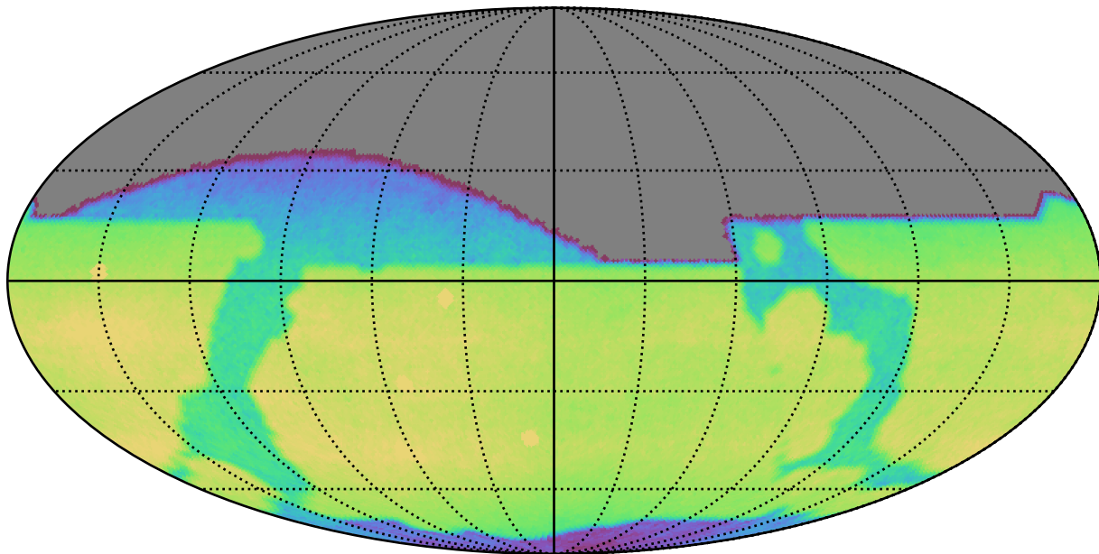
ddf_loaded_fl8_v3.4_10yrs All sky i band: CoaddM5
