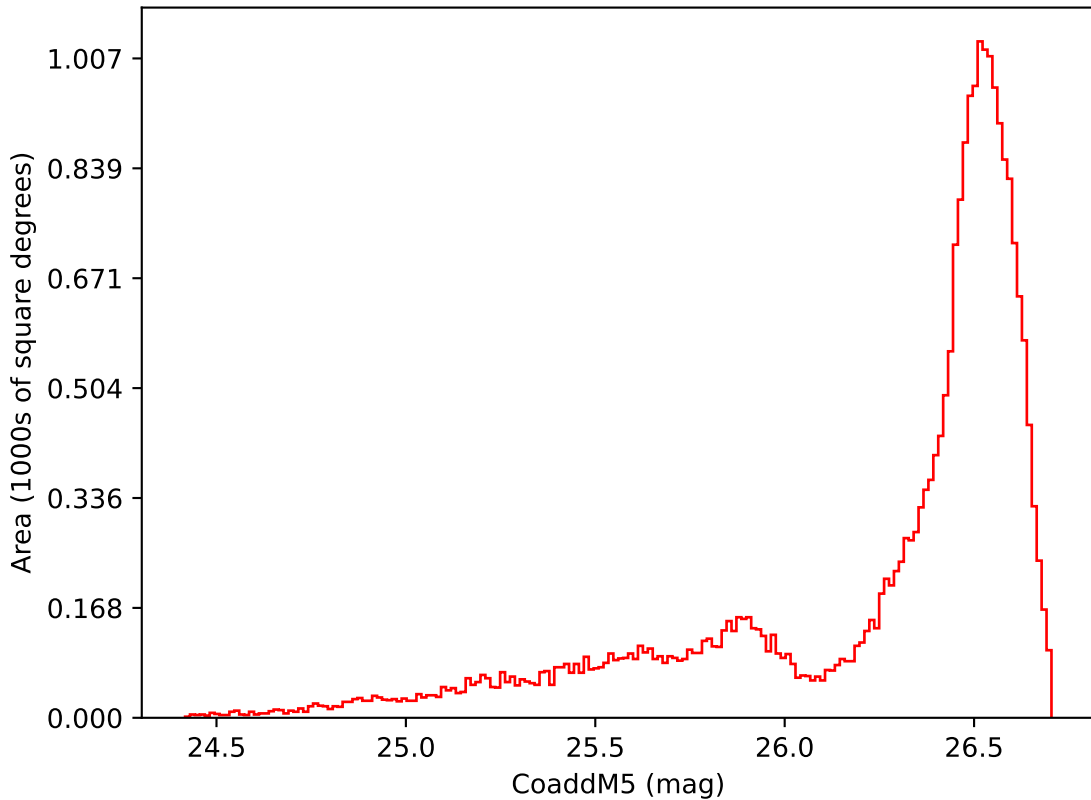
ddf_loaded_fl8_v3.4_10yrs All sky i band: CoaddM5
