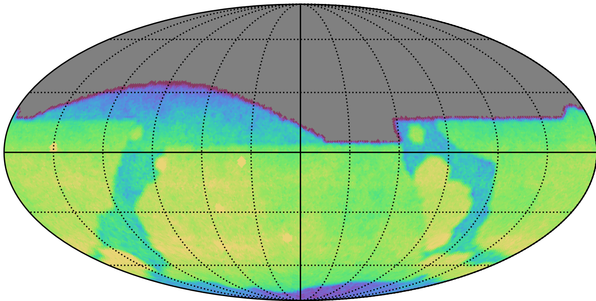
ddf_loaded_fl8_v3.4_10yrs All sky g band: CoaddM5
