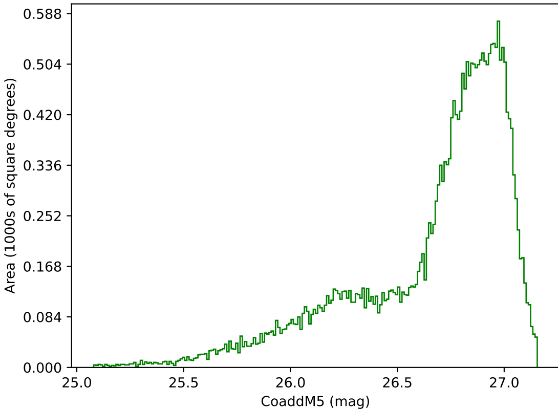
ddf_loaded_fl8_v3.4_10yrs All sky g band: CoaddM5
