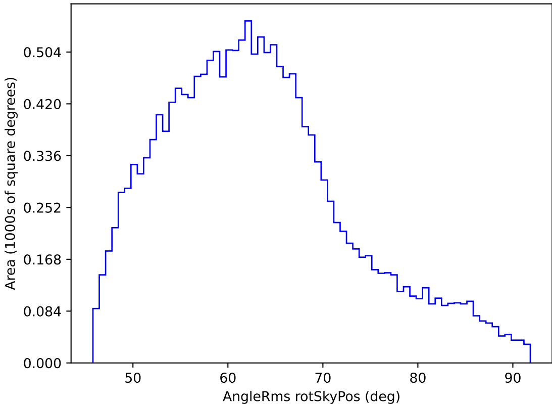
ddf_loaded_fl8_v3.4_10yrs WFD y band: AngleRms rotSkyPos
