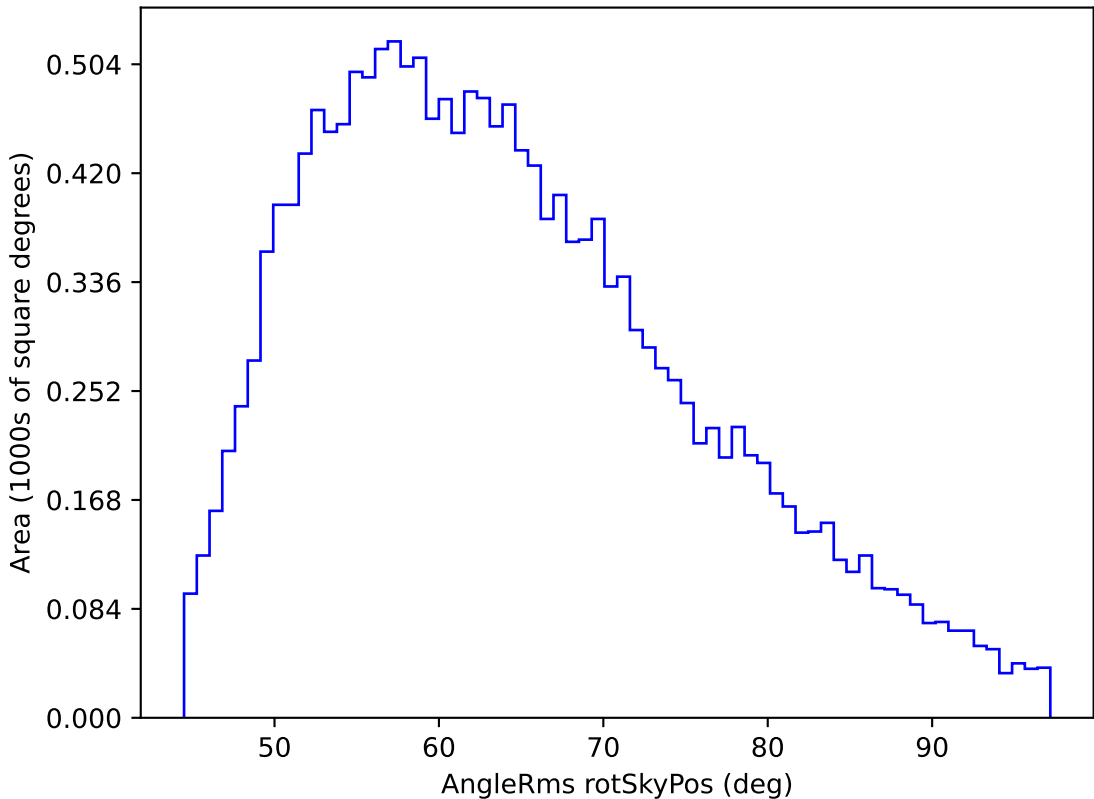
ddf_loaded_fl8_v3.4_10yrs WFD u band: AngleRms rotSkyPos
