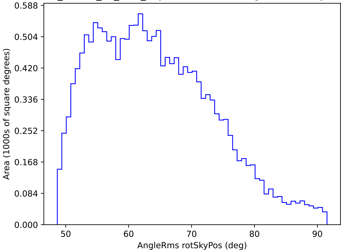
ddf_loaded_fl8_v3.4_10yrs WFD i band: AngleRms rotSkyPos
