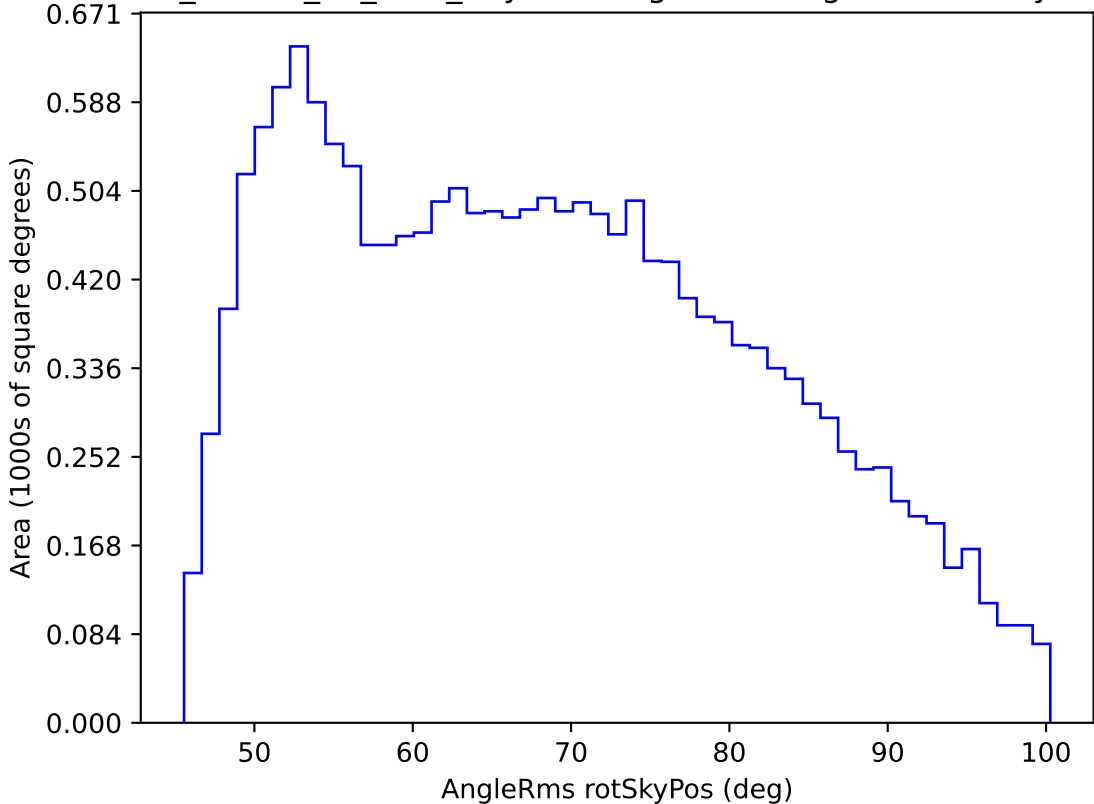
ddf_loaded_fl8_v3.4_10yrs WFD g band: AngleRms rotSkyPos
