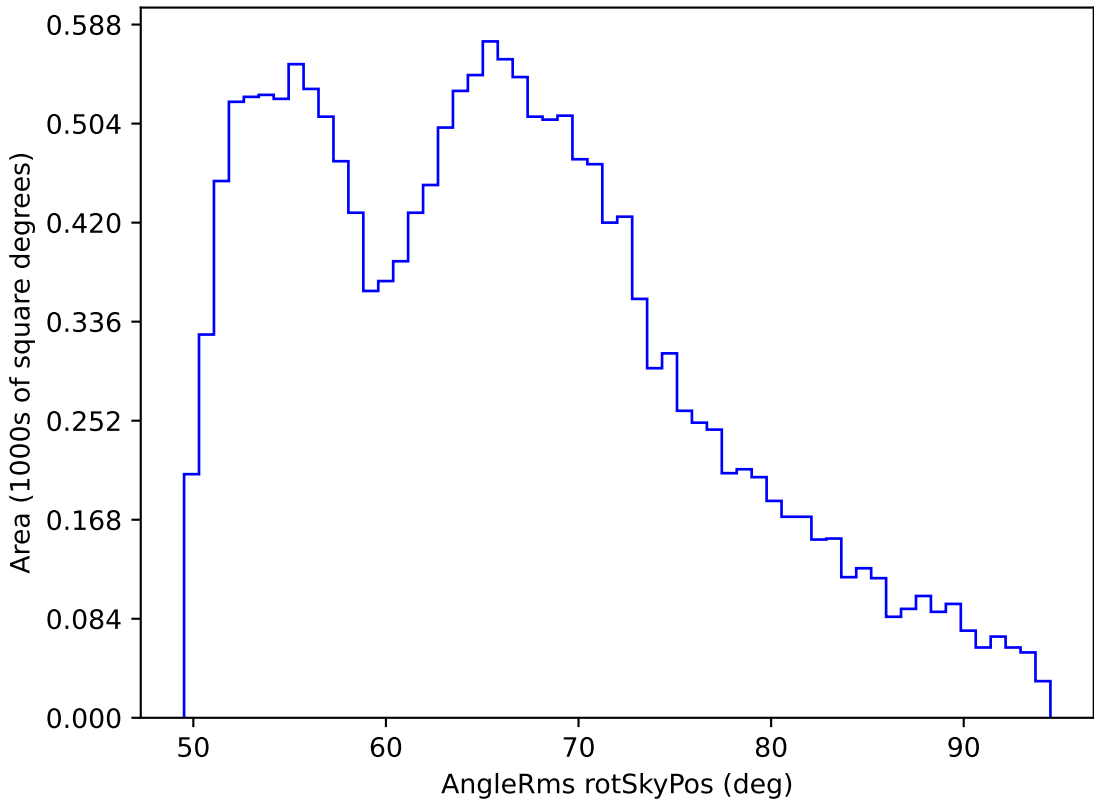
ddf_loaded_fl8_v3.4_10yrs WFD all bands: AngleRms rotSkyPos
