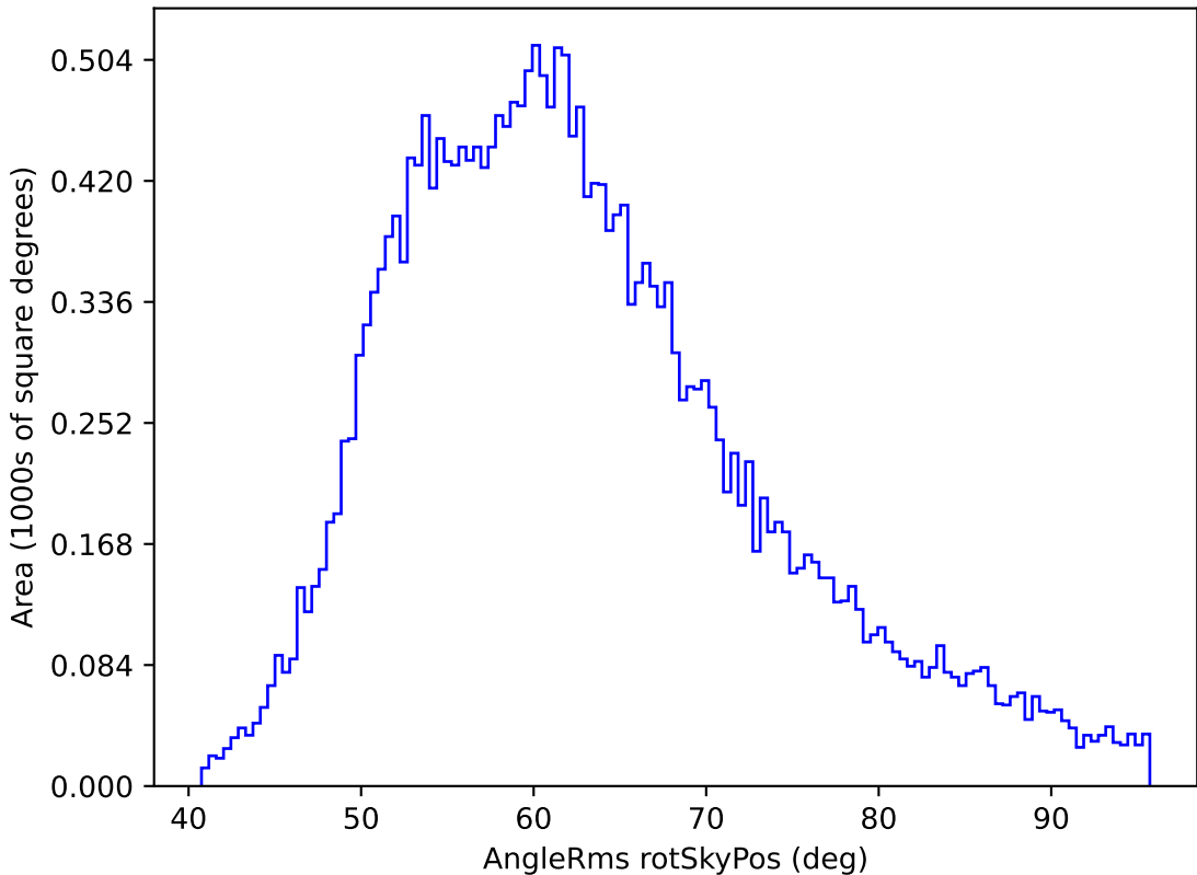
ddf_loaded_fl8_v3.4_10yrs All sky z band: AngleRms rotSkyPos
