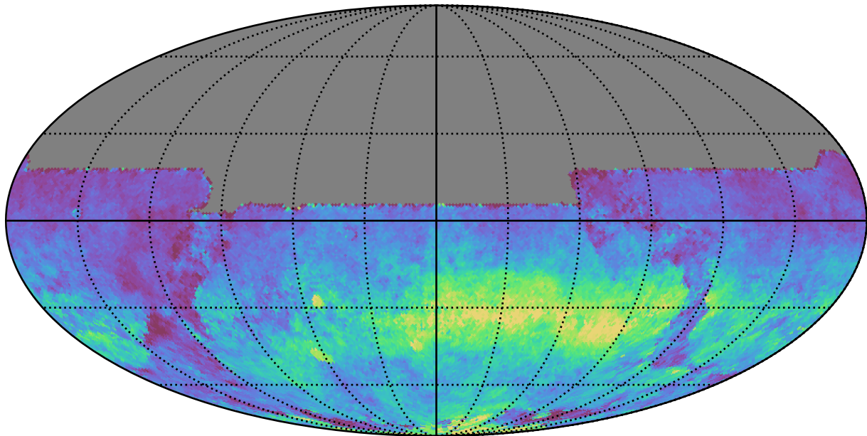
ddf_loaded_fl8_v3.4_10yrs All sky y band: AngleRms rotSkyPos
