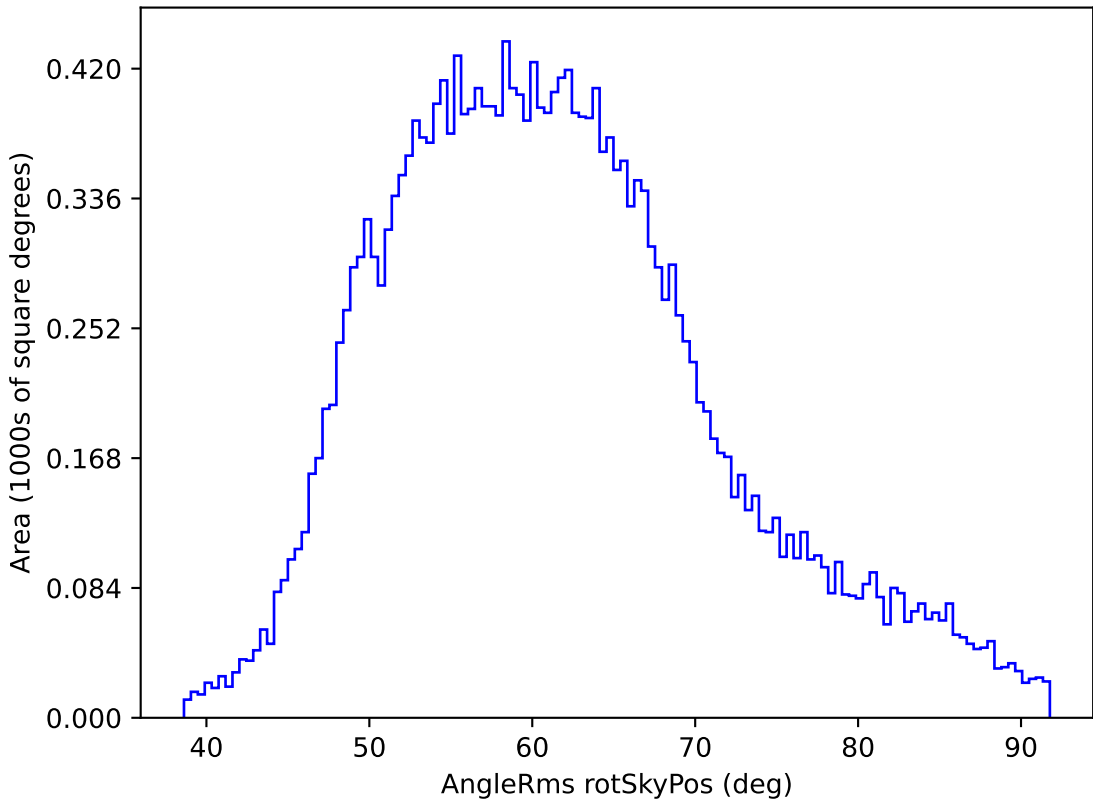
ddf_loaded_fl8_v3.4_10yrs All sky y band: AngleRms rotSkyPos
