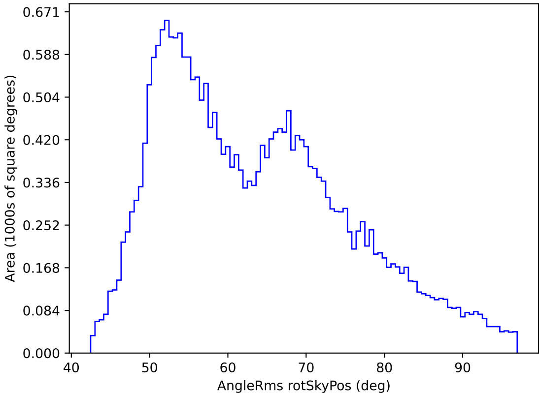
ddf_loaded_fl8_v3.4_10yrs All sky r band: AngleRms rotSkyPos
