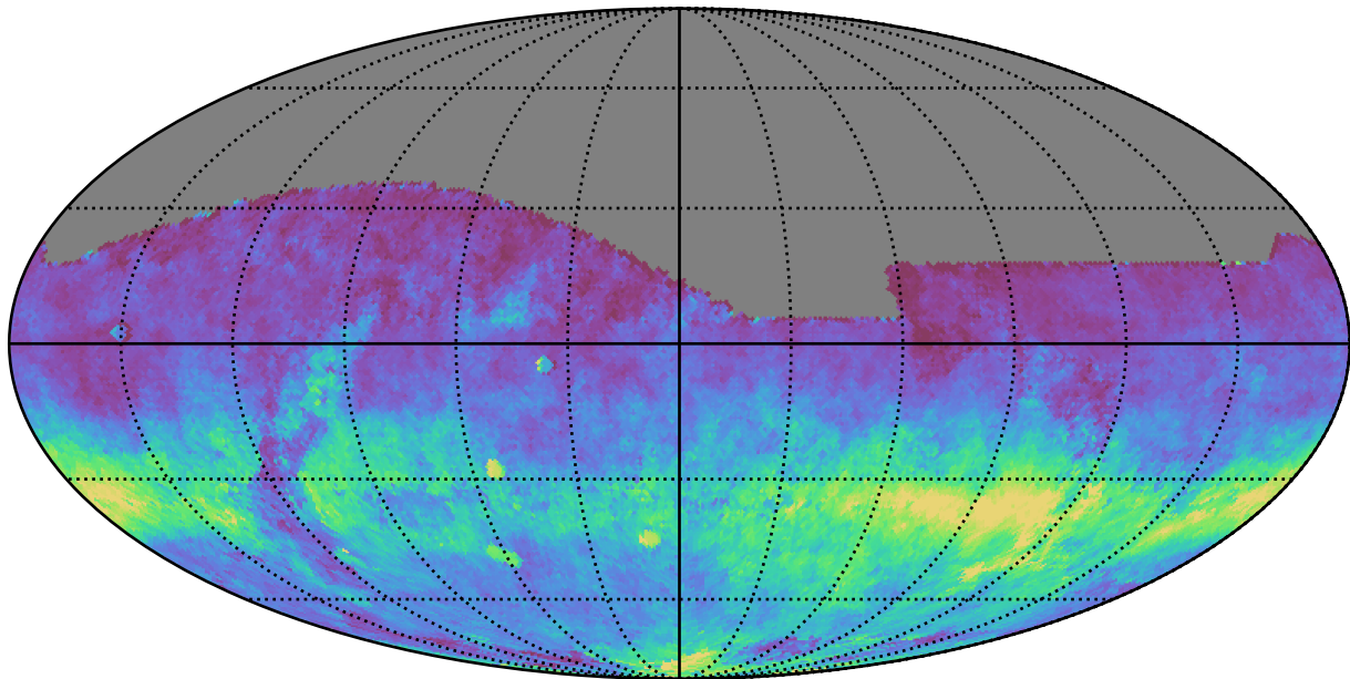
ddf_loaded_fl8_v3.4_10yrs All sky i band: AngleRms rotSkyPos
