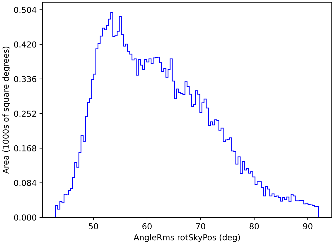
ddf_loaded_fl8_v3.4_10yrs All sky i band: AngleRms rotSkyPos
