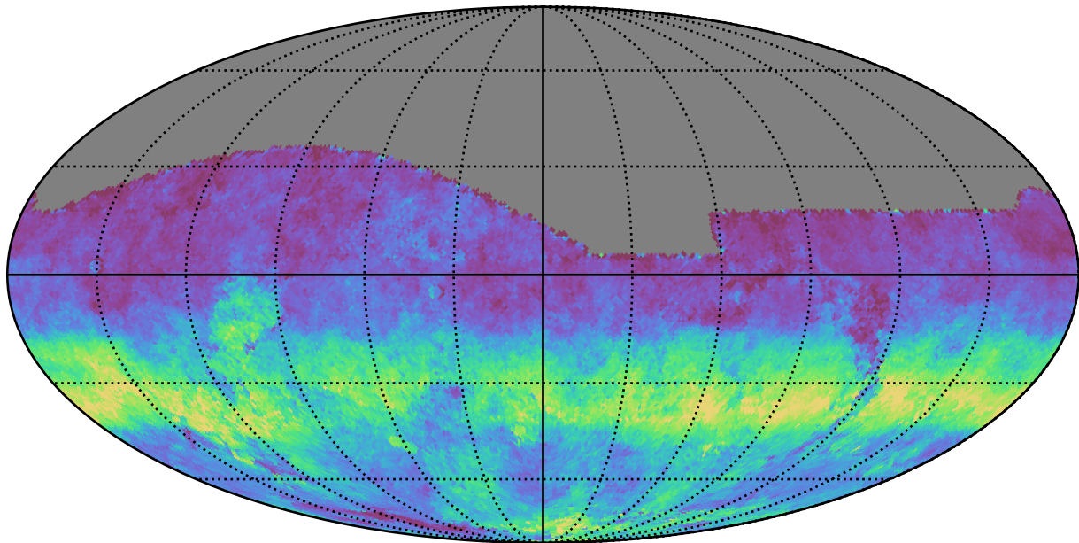
ddf_loaded_fl8_v3.4_10yrs All sky g band: AngleRms rotSkyPos
