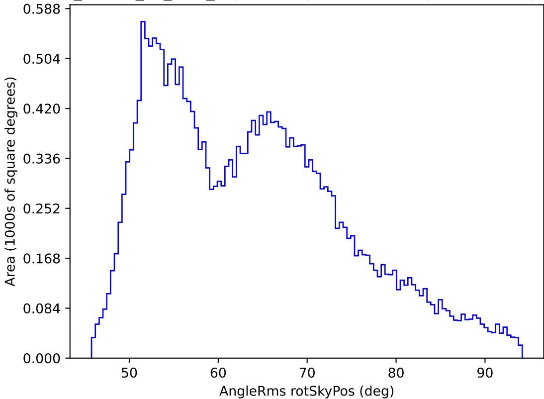
ddf_loaded_fl8_v3.4_10yrs All sky all bands: AngleRms rotSkyPos
