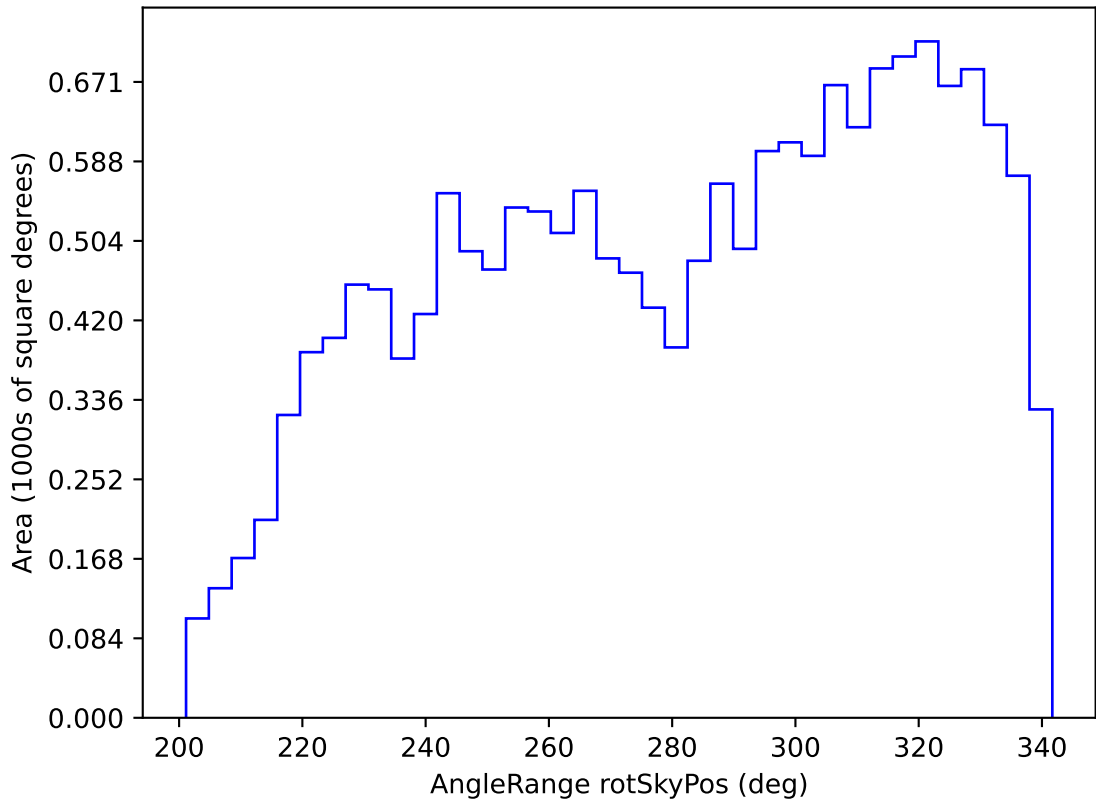
ddf_loaded_fl8_v3.4_10yrs WFD z band: AngleRange rotSkyPos
