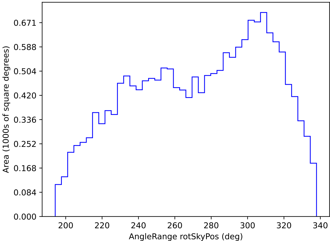
ddf_loaded_fl8_v3.4_10yrs WFD y band: AngleRange rotSkyPos
