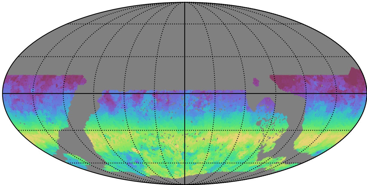
ddf_loaded_fl8_v3.4_10yrs WFD r band: AngleRange rotSkyPos
