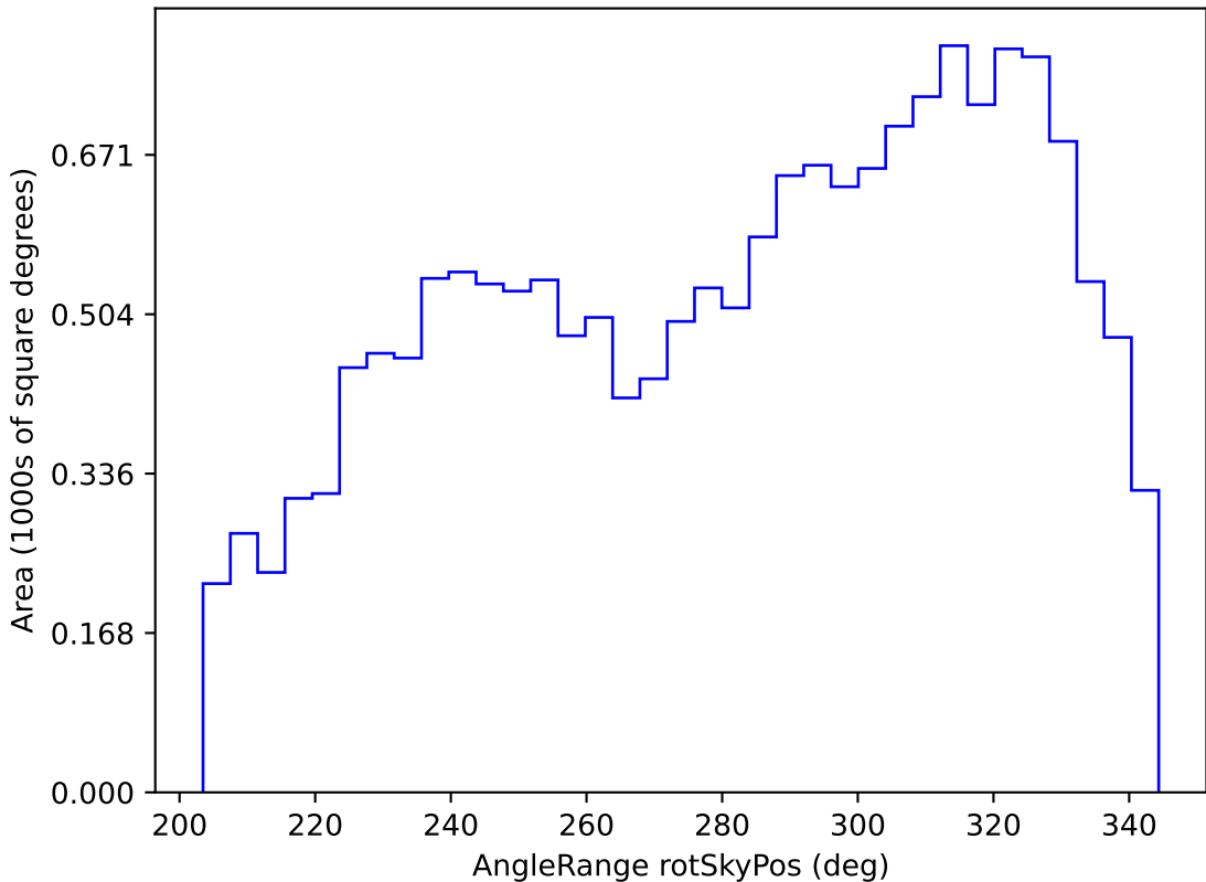
ddf_loaded_fl8_v3.4_10yrs WFD r band: AngleRange rotSkyPos
