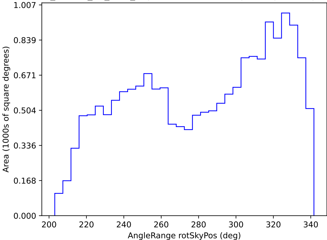
ddf_loaded_fl8_v3.4_10yrs WFD i band: AngleRange rotSkyPos
