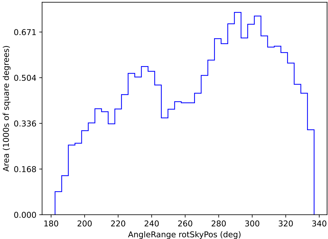
ddf_loaded_fl8_v3.4_10yrs WFD g band: AngleRange rotSkyPos
