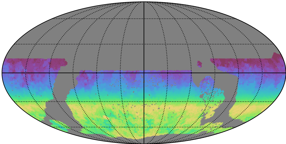
ddf_loaded_fl8_v3.4_10yrs WFD all bands: AngleRange rotSkyPos
