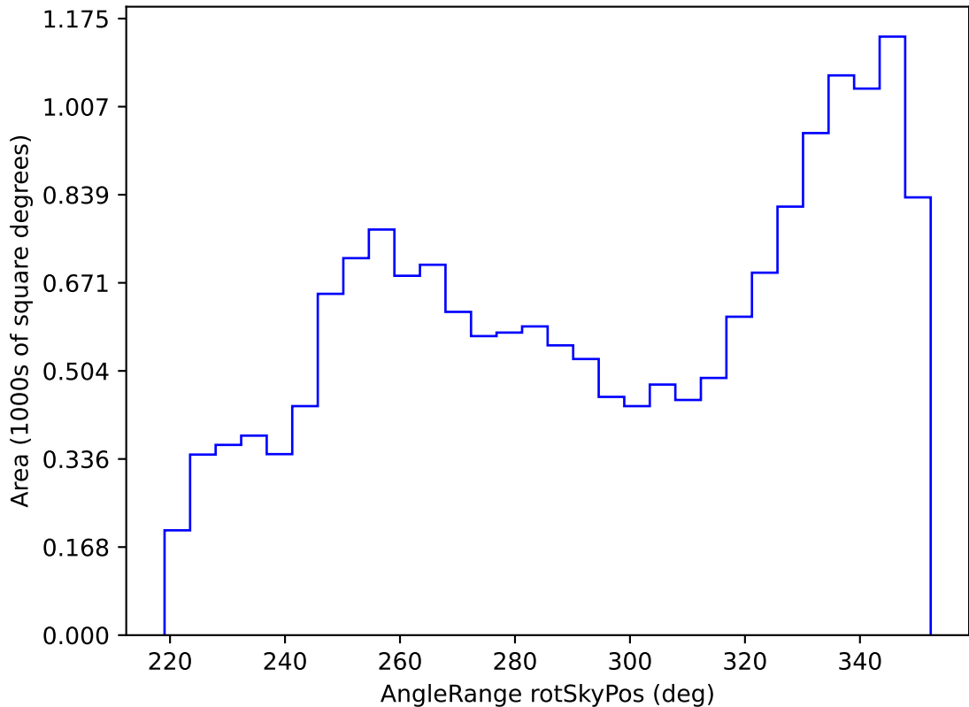
ddf_loaded_fl8_v3.4_10yrs WFD all bands: AngleRange rotSkyPos
