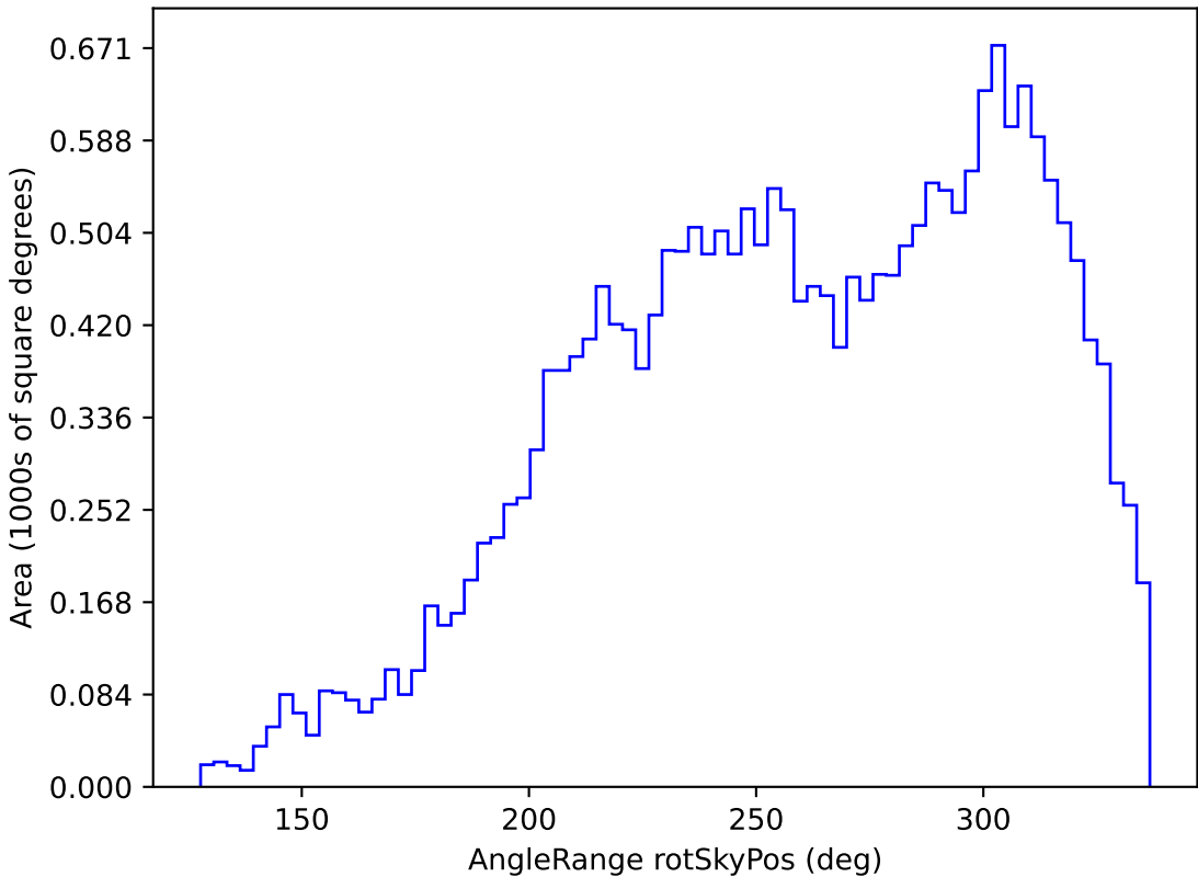
ddf_loaded_fl8_v3.4_10yrs All sky y band: AngleRange rotSkyPos
