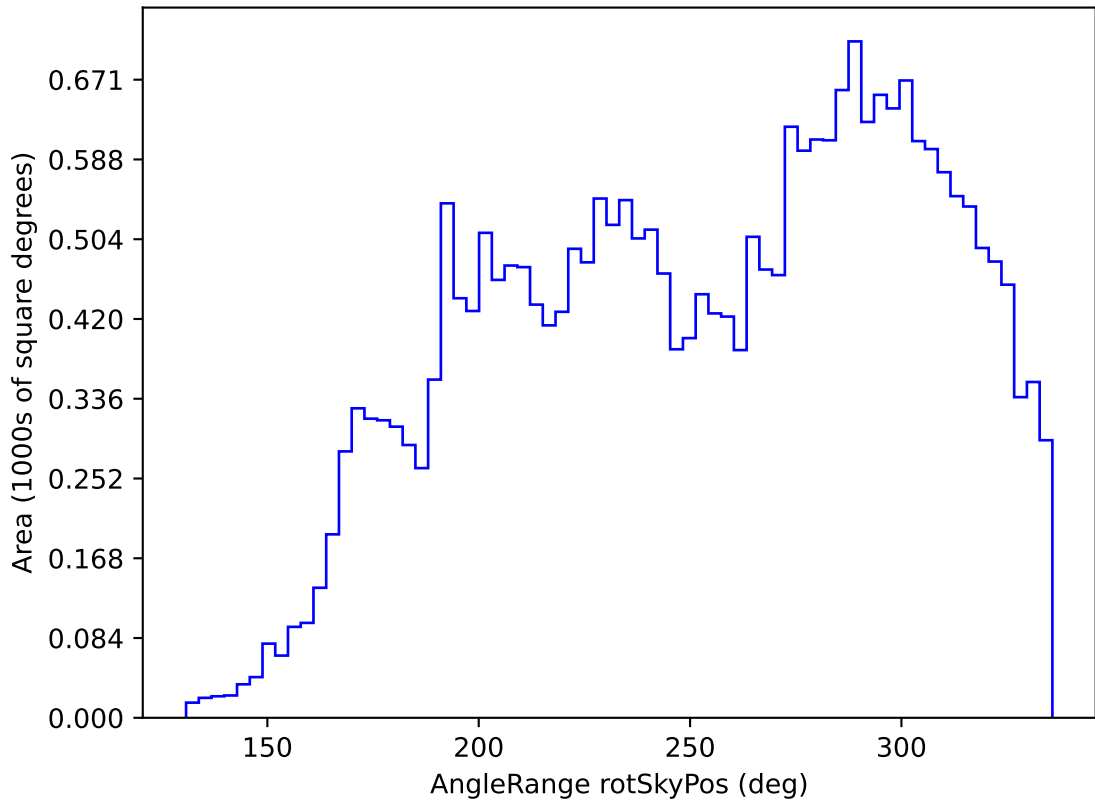
ddf_loaded_fl8_v3.4_10yrs All sky g band: AngleRange rotSkyPos
